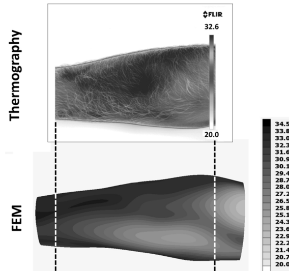
Fig. 7. Comparison of numerical solution and measurements
