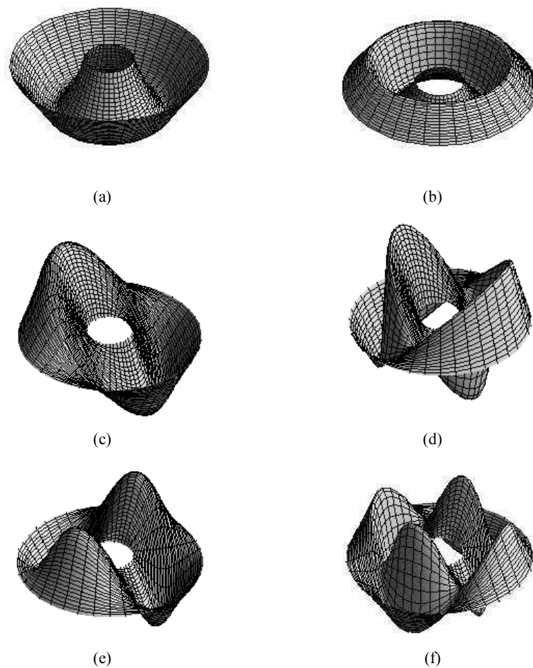
Fig. 2. Mode shapes for an annular membrane: a) \Omega_{01}=1.01416 , b) \Omega_{02}=2.86149 , c) \Omega_{11}=1.09474 , d) \Omega_{12}=2.90734 , e) \Omega_{21}=1.29468 , f) \Omega_{22}=3.03193
