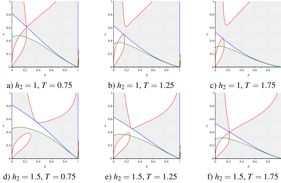
Fig. 4. Modulational stability diagram of wave packets in the HS-La system
