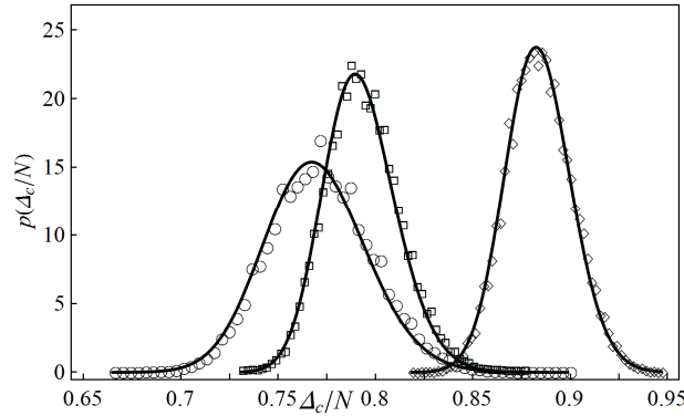
Fig. 5. Empirical probability density functions of the \Delta_c / N in an array with: 40 \times 40 (uniform distribution, circles), 80 \times 80 (uniform distribution, squares) and 80 \times 80 pillars (Weibull distribution with index \rho = 2 , diamonds). The solid lines represent skew-normally distributed \Delta_c / N with parameters computed from the samples
