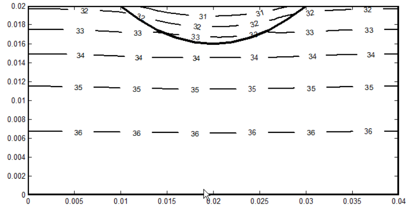
Fig. 3. Temperature distribution
