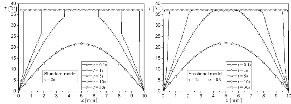
Fig. 1. Comparison of analytical solution of equation (7) over space for \tau = 2 s (left-side) with numerical solution of equation (6) over space for \tau = 2 s and \alpha = 0.9 (right-side)
